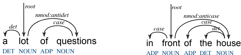
Figure 7. Enhanced analysis A for a lot (of) and in front (of)
